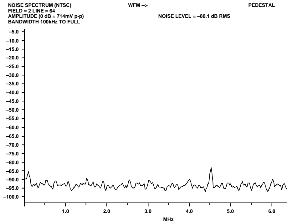
Figure 85. NTSC SNR Pedestal Measurement
