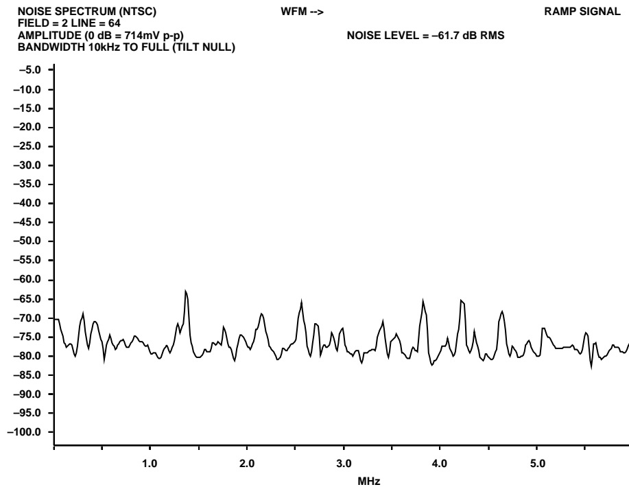
Figure 86. NTSC SNR Ramp Measurement
